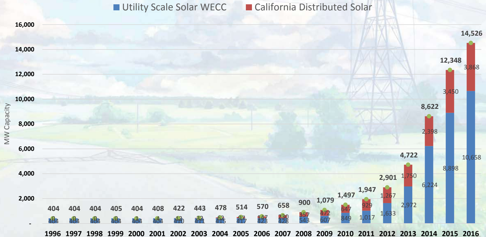
WECC Utility Scale Solar and California Distributed Solar
